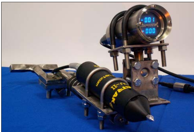
Deep-C-Meter kit includes an ROV II probe (pictured here on the ROV T-Handle)
